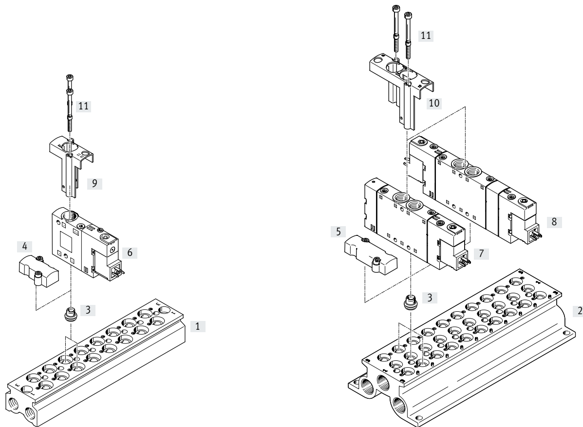
Example of manifold assembly – CPE18
