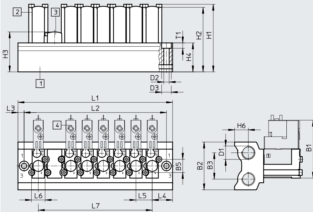
[1] Manifold block
