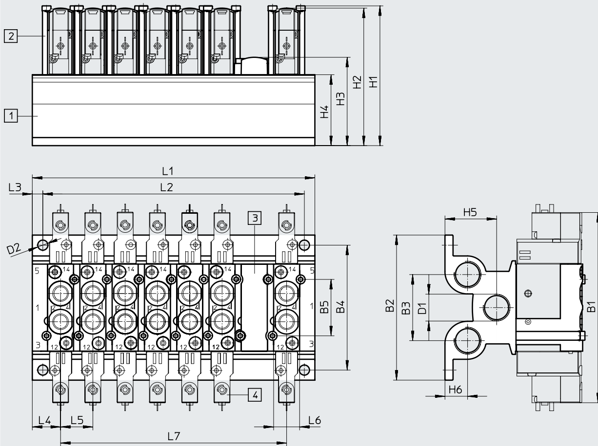
[1] Manifold block [2] Retaining bracket [3] Cover plate [4] Valves
